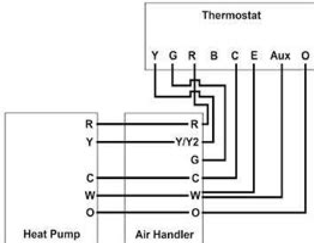
Wiring Diagram for Air Handler with Electric Resistance Heat and Heat Pump
