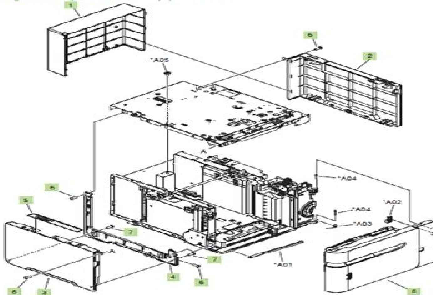
Figure 8-19 Optional 1,500-sheet paper feeder covers
