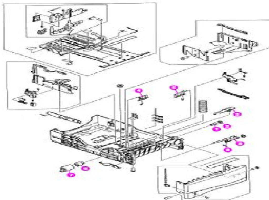
Figure 137. 500-sheet tray
