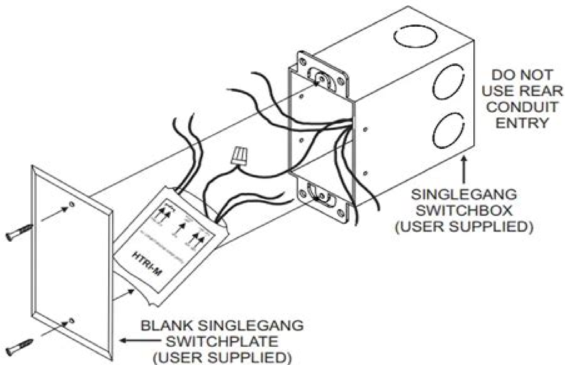
Figure 4 Mounting the HTRI-M
