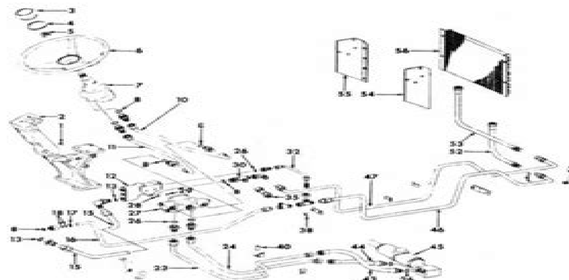
Fig. IH1308A — Schematic view showing the general lay-out of components and tubing for the full time (Hydrostatic) power steering used on International 504 and 2504 tractors.
