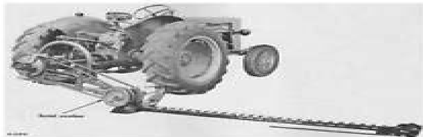
Fig. 100 Balanced Mower (PowerCut Model)
