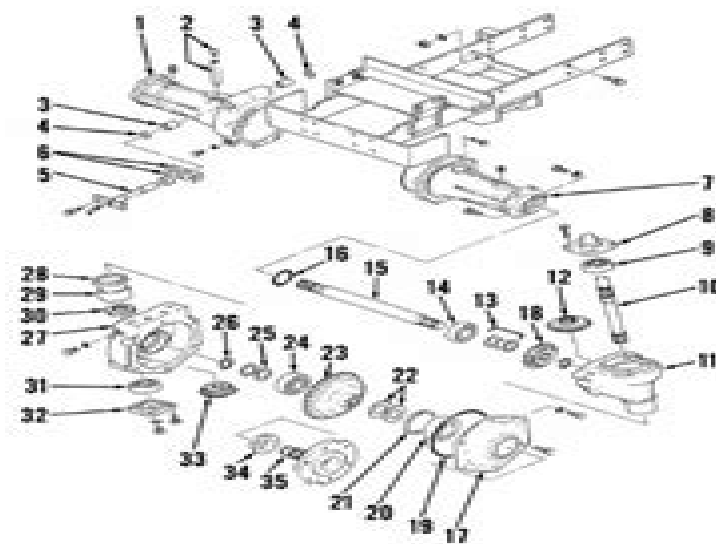
Fig. 9—Exploded view of four-wheel drive front axle assembly available on Models 244 and 254.
