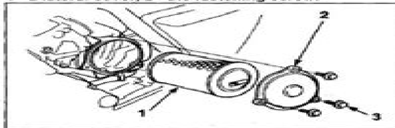
1 - a filtering element, 2 - a cover of the case of the air filter.
