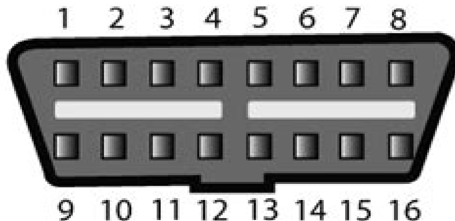
J1962 Type B
