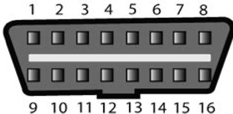
J1962 Type A
