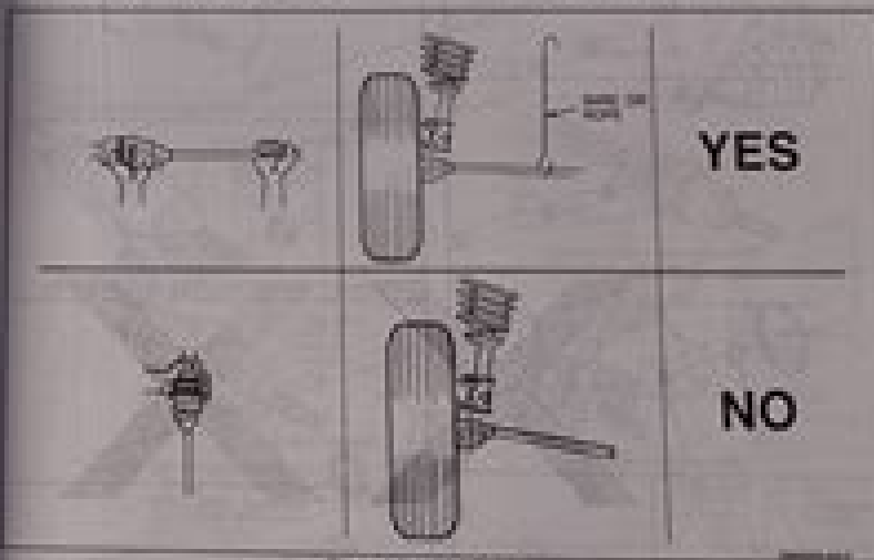
Figure 4 Drive Shaft Hanger
