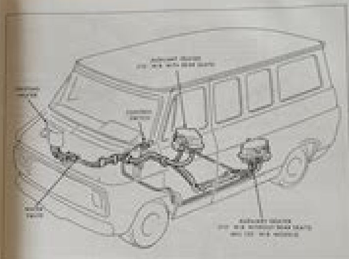
Fig. 15-Install the heater
