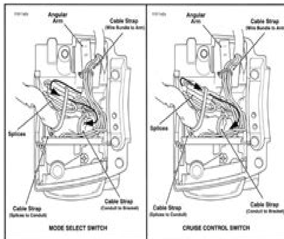
Figure 8-125. Lower Right Handstar Switch Housing (With Splices) - Classic/Lite Models
