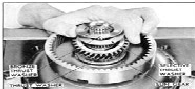
Fig. 167 Installing Sun Gear and Selective Washer for Front Unit End Clearance Check
