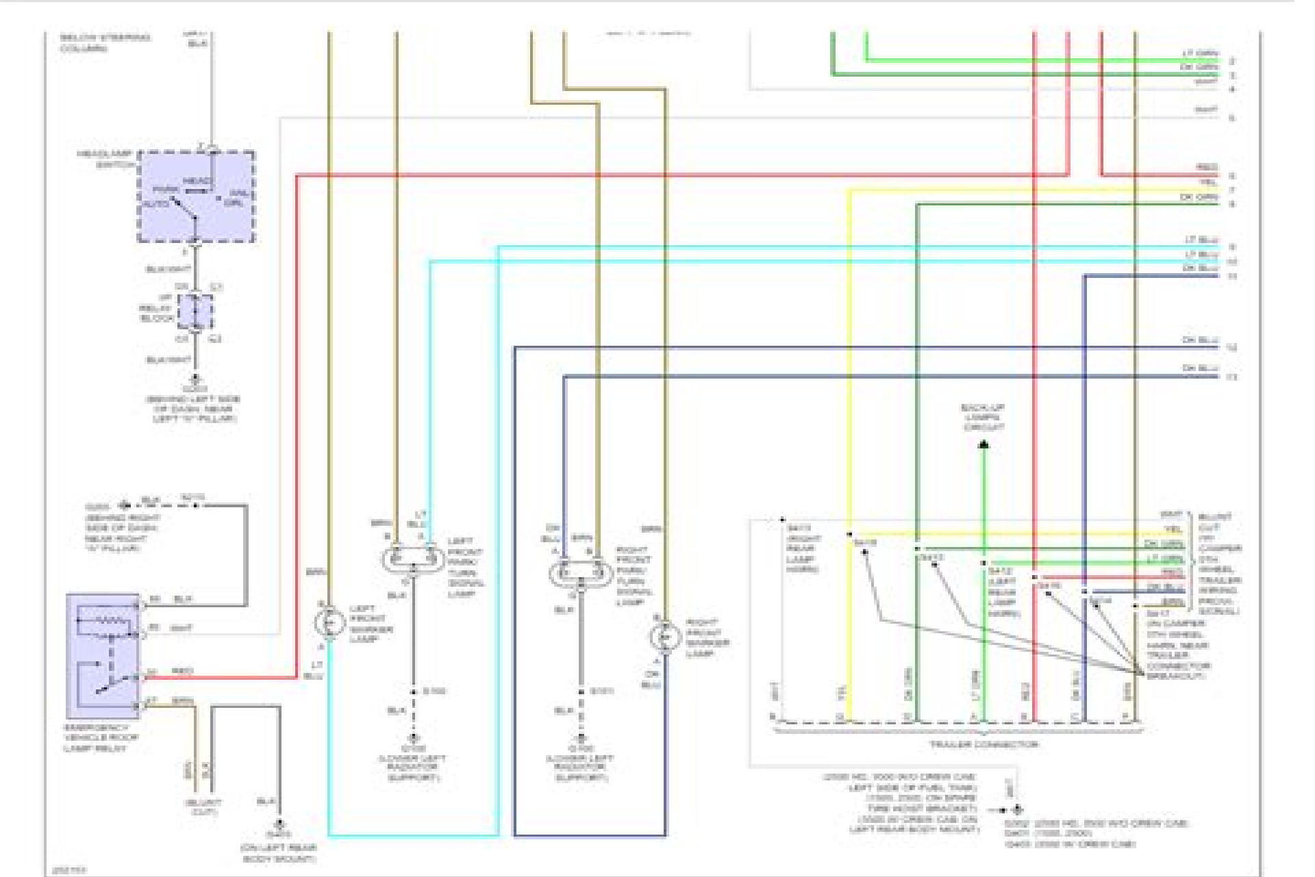
Fig 2: Exterior Lamps Circuit (1 of 3)
