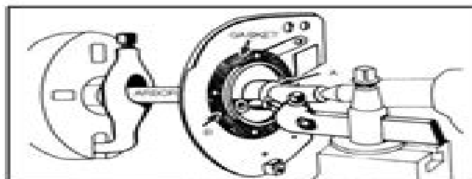
Fig. 892 – CORRECTING END PLAY
