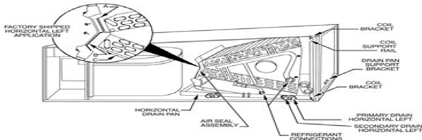
Fig. 3 - A-Coil in Horizontal-Left Application (Factory Ready FE4A Only)
