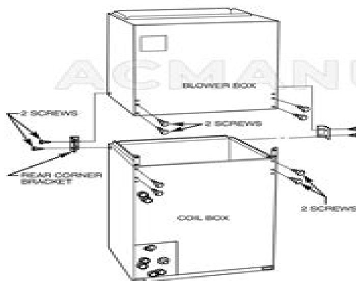
Fig. 4 - Modular Unit Assembly
