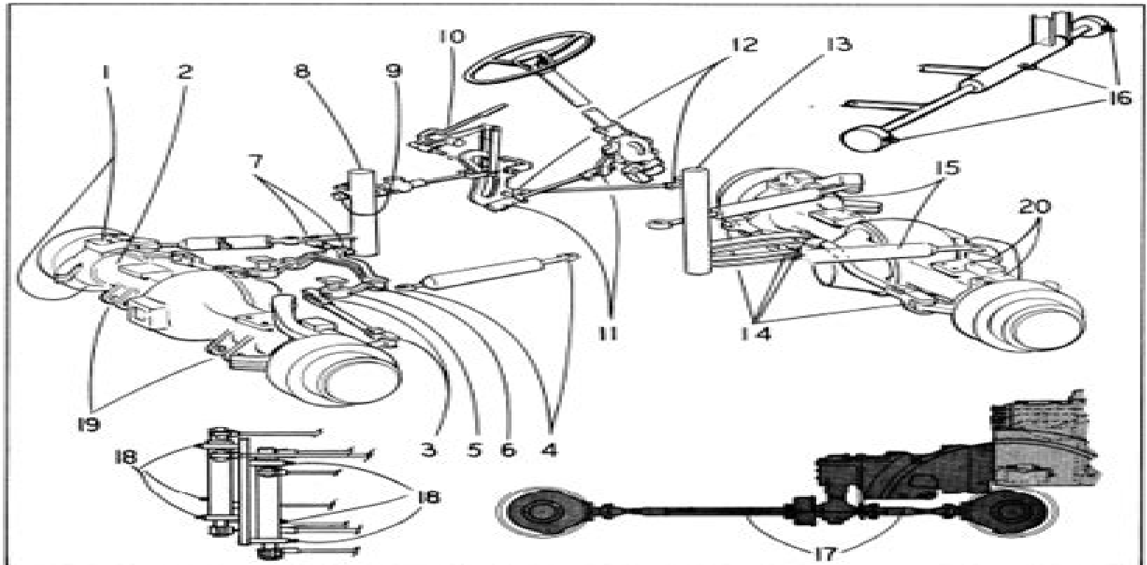
Figure 37. Chassis lubrication diagram
