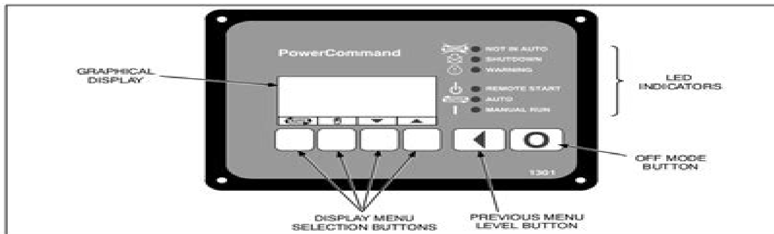
FIGURE 2-2. FRONT PANEL (WITH DISPLAY)
