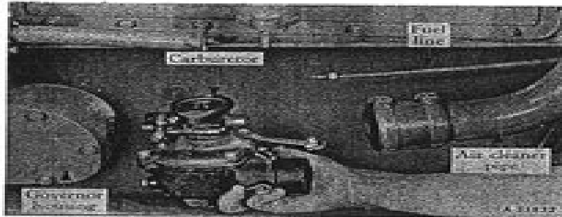
Illustr. 43 Removing the carburetor.
