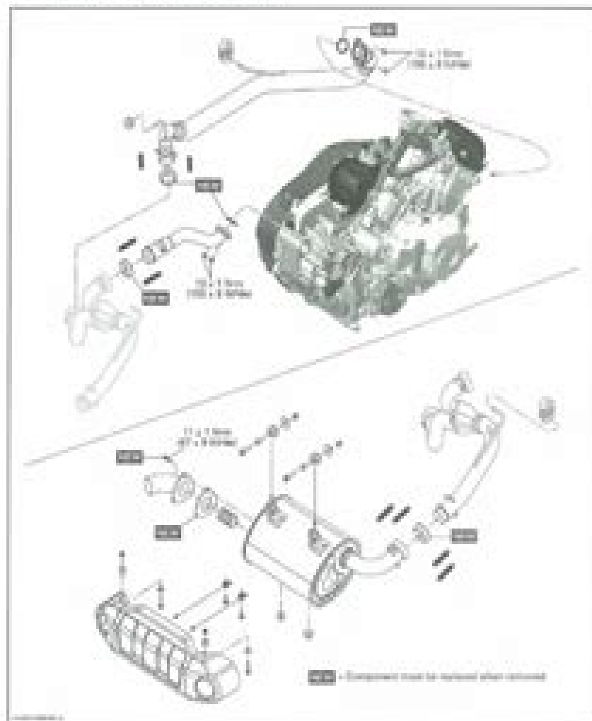
1. Exhaust system
