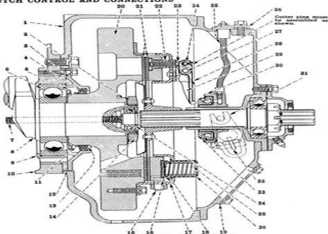
Clutch Control and Single Plate Clutch.
