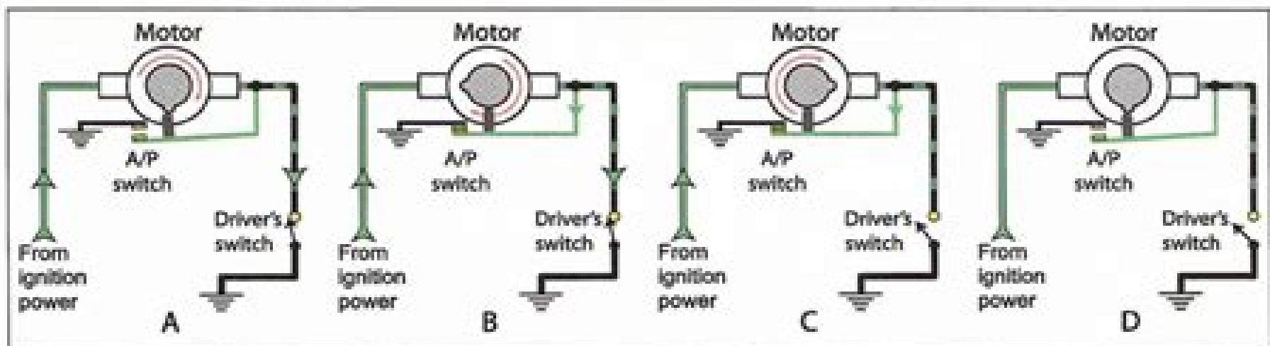
Figure 14.3. Operational sequence for the DR wiper motor auto-park mechanism.
