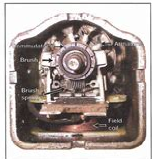
Figure 14.5. Open rear view of the DR wiper motor.
