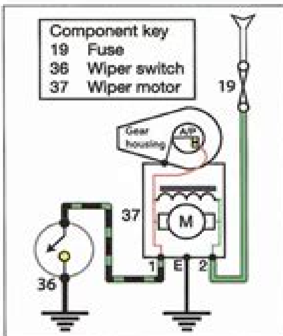
Figure 14.2. The DR wiper motor circuit.
