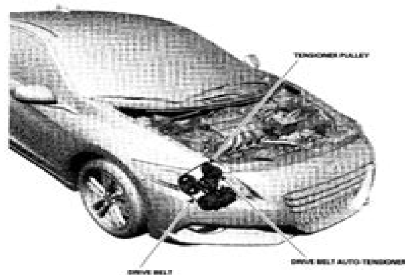
Fig. 2: Identifying Cooling System Components (2 Of 2) Courtesy of AMERICAN HONDA MOTOR CO., INC.
