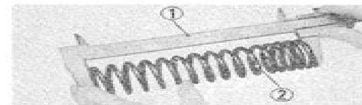
① Vernier caliper ② Front cushion spring Fig. 5-23. Measuring free length of cushion spring
