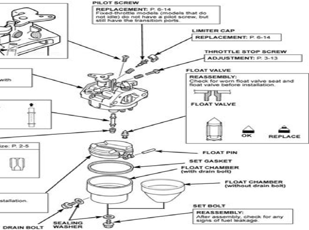
DRAIN BOLT
