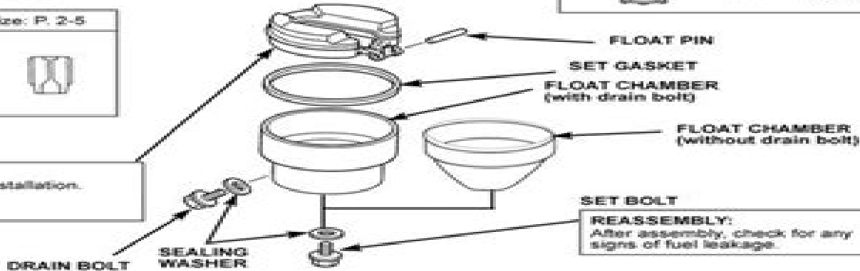
DRAIN BOLT
