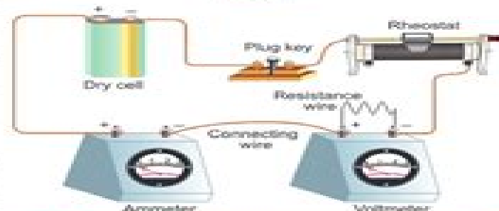
Fig. 4.3 Arrangement for studying the dependence of potential difference ( V ) across a metallic resistor on current ( I ) passing through it
