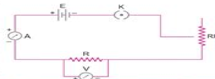
Fig. 4.2 Circuit diagram for studying the dependence of potential difference ( V ) across a metallic resistor on current ( I ) passing through it
