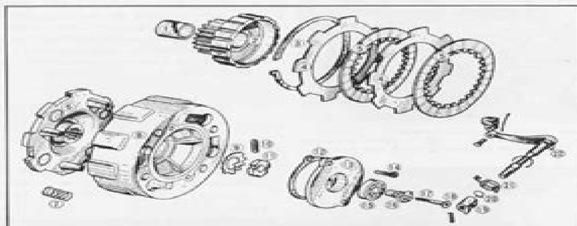
Fig. 3.64 Component parts of clutch: G 90, CL 90, CL 90 L, G0 90
