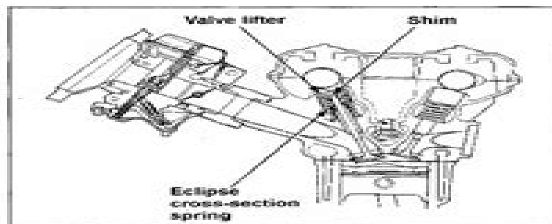
Eclipse cross-section
