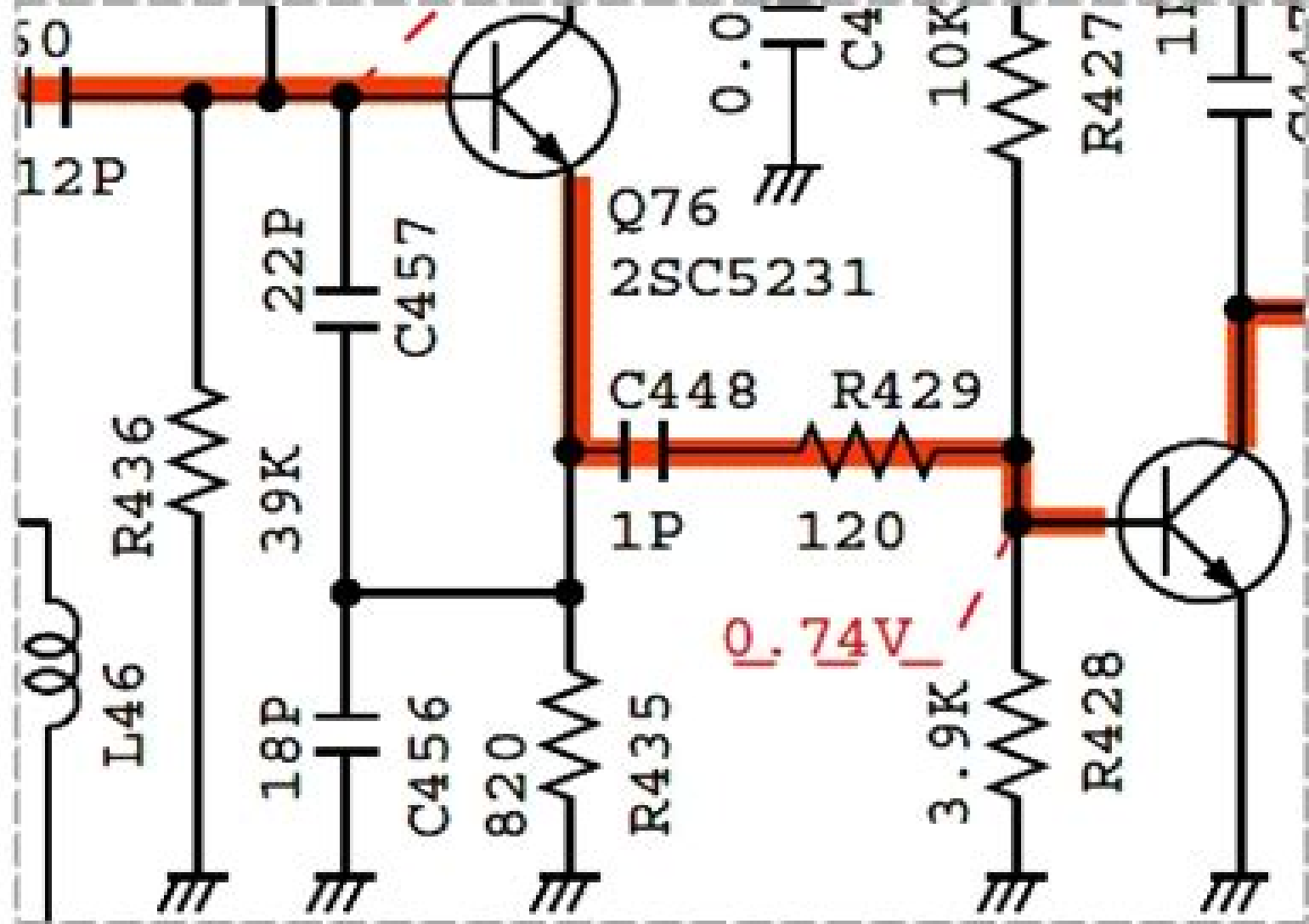
Preview: ICOM IC-V85 /E /T schematic diagram
